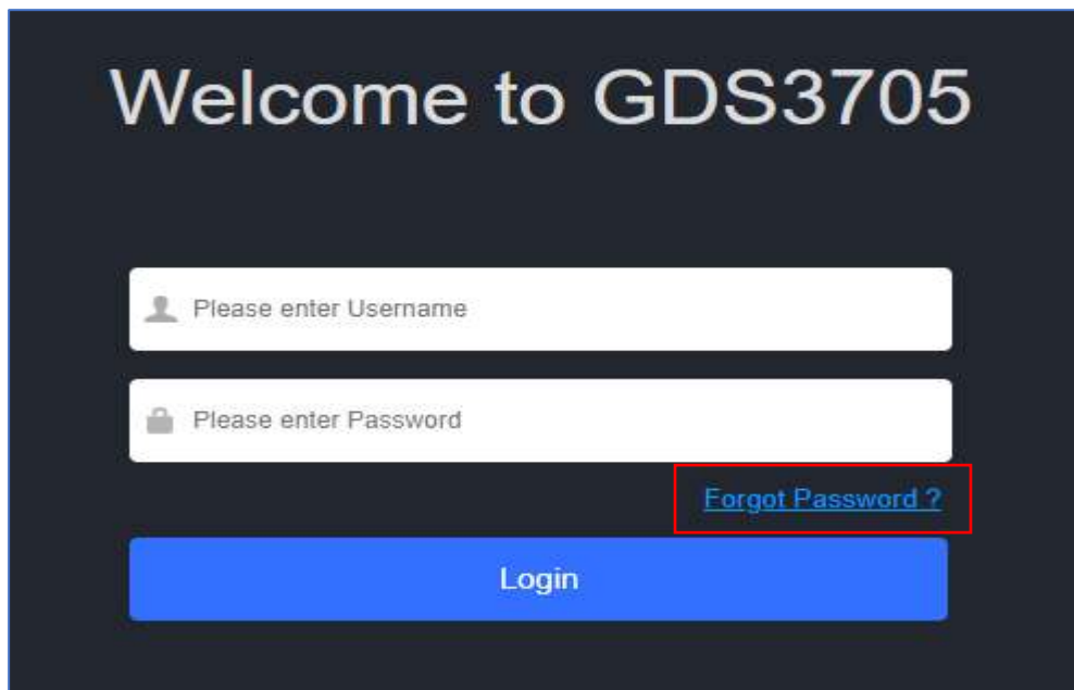
Figure 60: Recover Password
