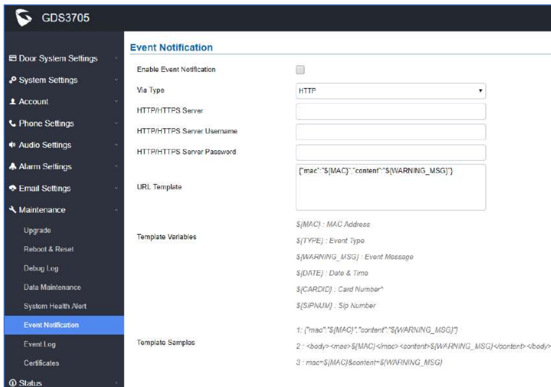
Figure 82: Event Notification
